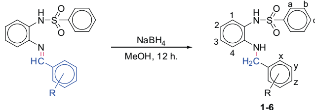
Fig. 1. Synthesis of the ligands together with NMR numbering scheme.
